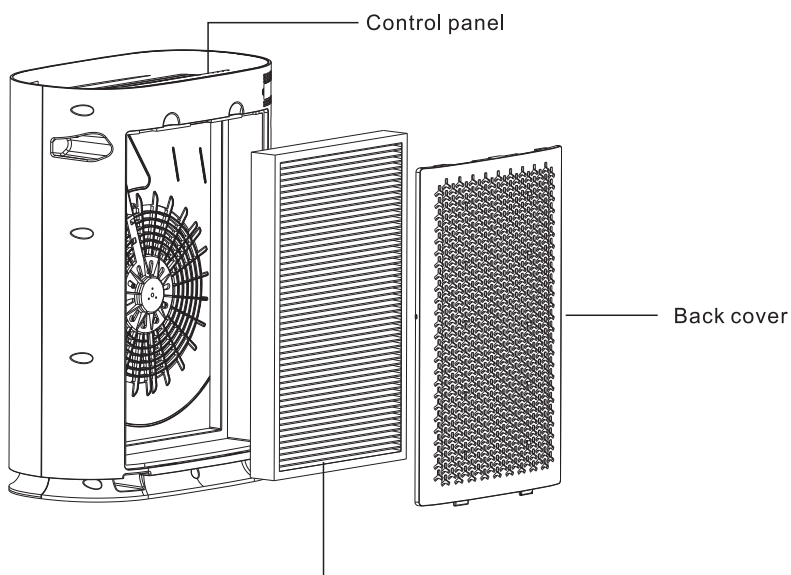
3 in 1 filter ( pre-filter + HEPA H13 filter + Active carbon filter)
